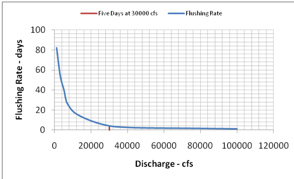
Figure 1. Residence time for Conowingo Reservoir
