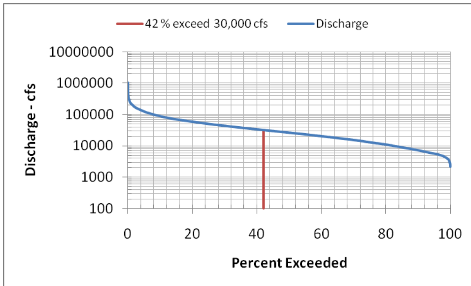
Figure 2. Flow duration curve for the Susquehanna River at Marietta, Pennsylvania
