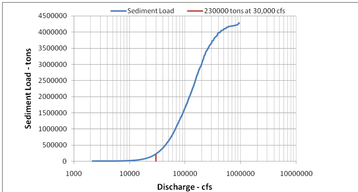
Figure 4. Annual cumulative sediment yield for the lower Susquehanna River
