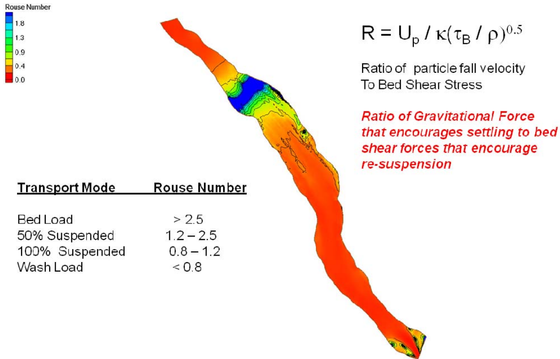
Figure 6. Rouse Number calculation for a medium silt sediment particle at 30,000
