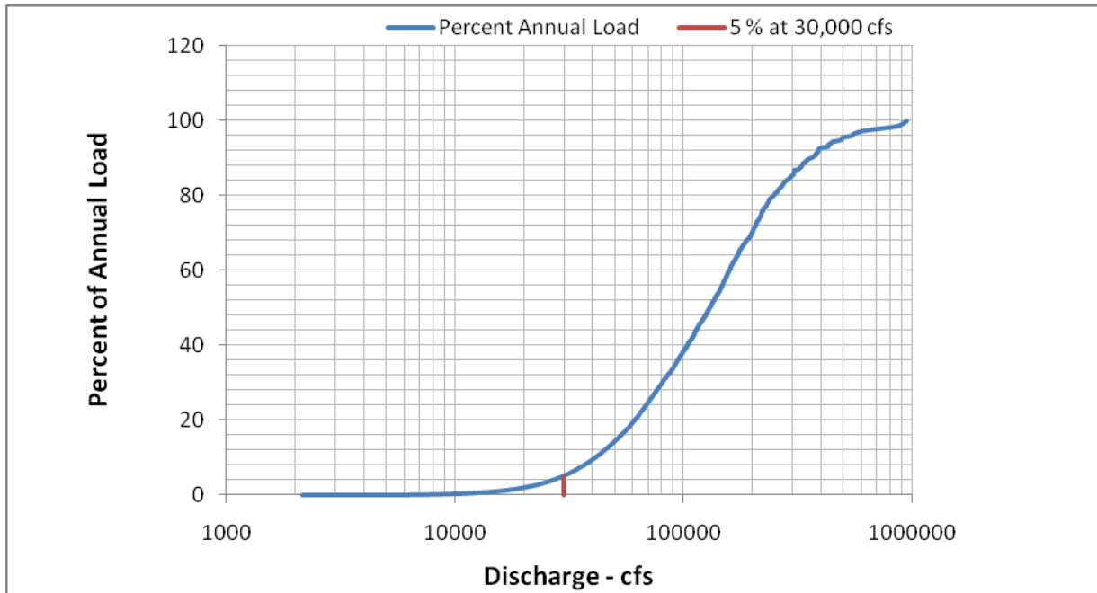
Figure 5. Percent of average annual yield for the lower Susquehanna River
