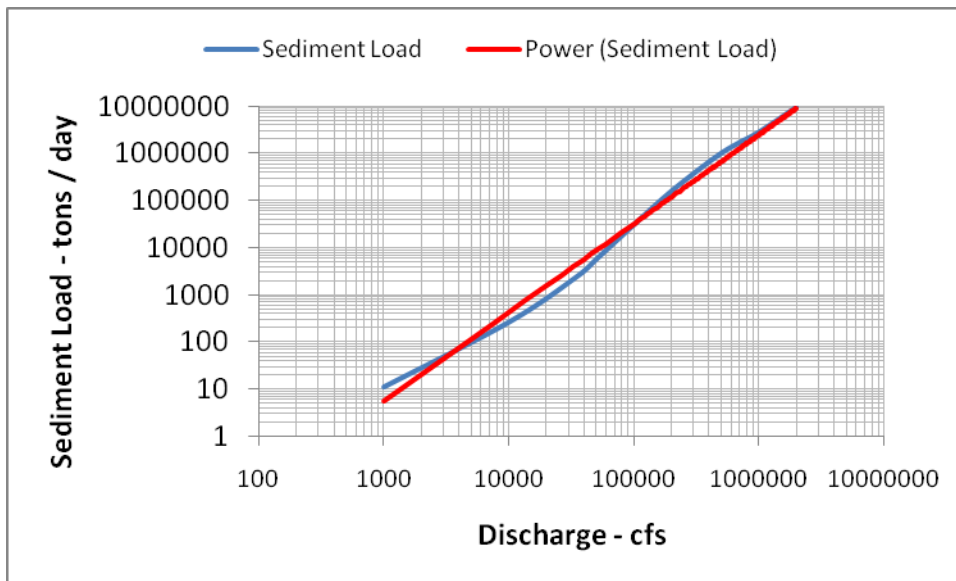
Figure 3. Sediment rating curve for the lower Susquehanna River
