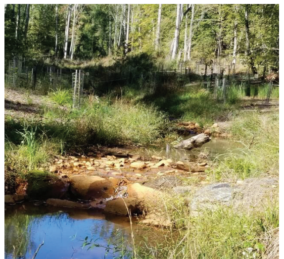
Step pools and planted vegetation in Flat Creek (2021).
